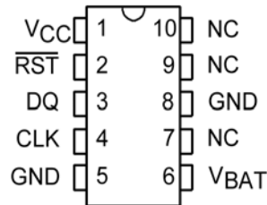
10-Pin DIP (300mil) See Mech. Drawings Section
